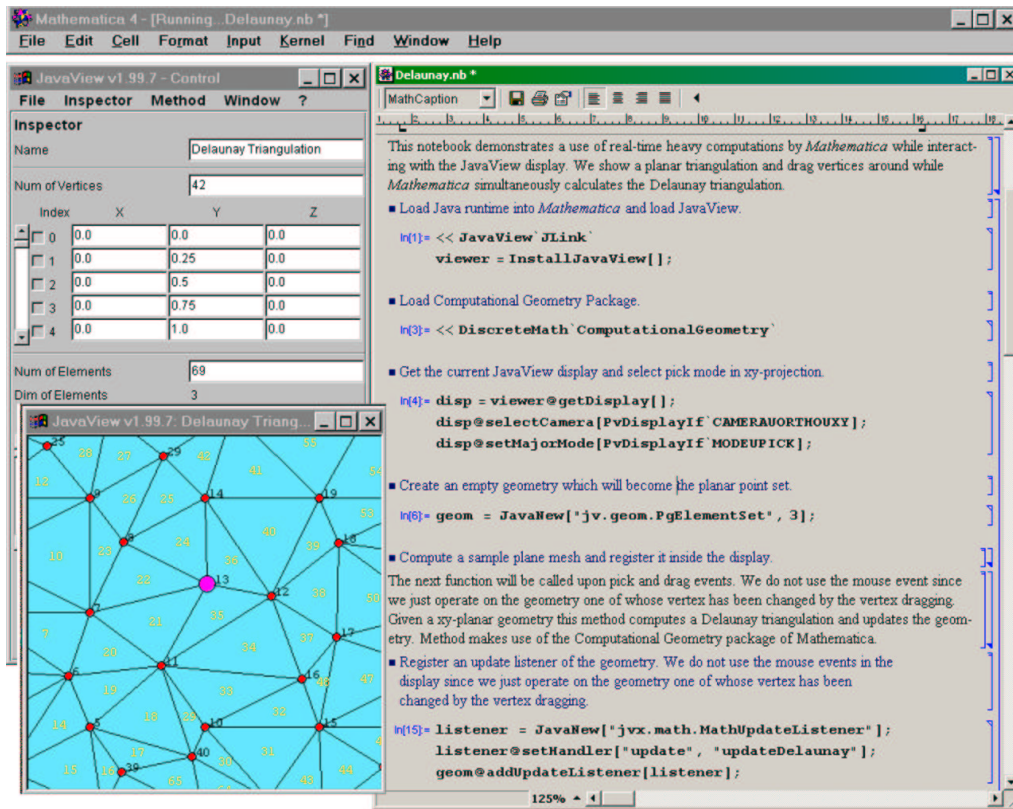
Fig. 2. Link Mathematica and JavaView via J/Link.
